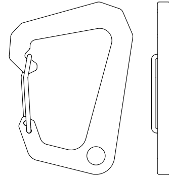
ASSEMBLY VIEW SCALE 1:1
