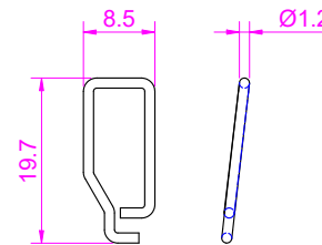
SPRING
