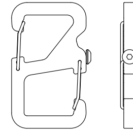
ASSEMBLY VIEW
